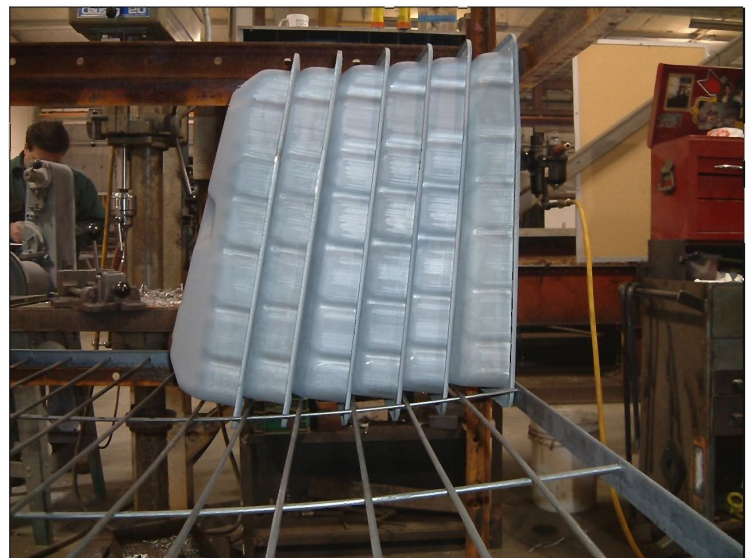
Parts fixture.
